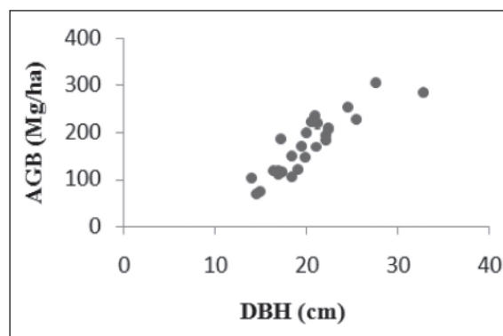
Fig. 2. Scatter plot between DBH and AGB (n=25).
