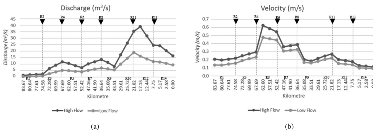
FIGURE 4. (a) Discharge ( \text{m}^3/\text{s} ) measurement at Sungai Langat and low flow scenario Q_{7,100} and (b) Velocity ( \text{m/s} ) of high and low flow scenario Q_{7,100}
