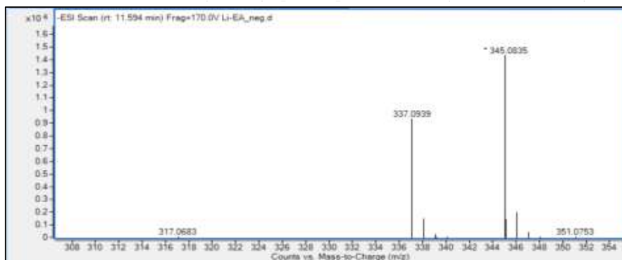
FIGURE 16. Fragmentation pattern from the MS/MS spectrum of the major peak with m/z value 345.0835
