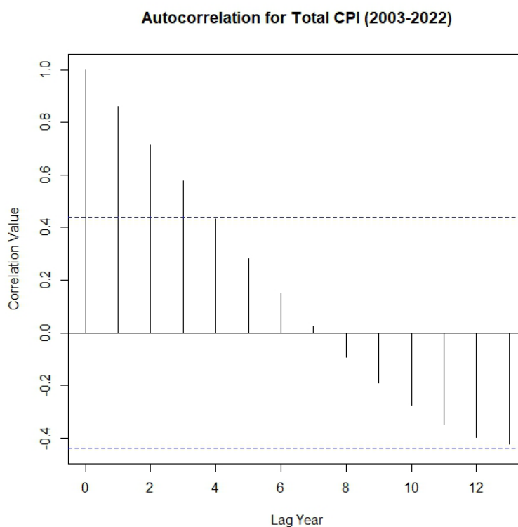
FIGURE 3. ACF plot for total CPI (2003–2022)
