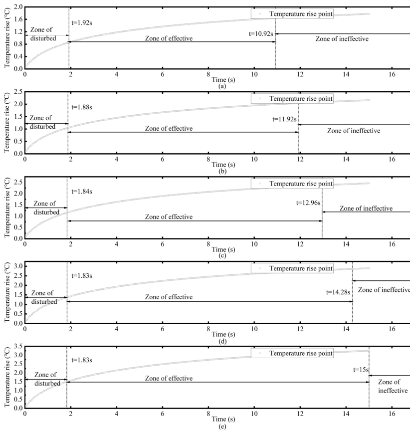
FIGURE 5. Variation of measurement intervals division with power (a) 2.1W , (b) P=2.5W , (c) P=3W , (d) P=3.5W , and (e) P=4.0W
