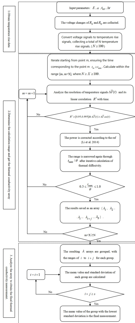
FIGURE 3. Flow chart of automatic algorithm for measuring thermal conductivity with TPS
