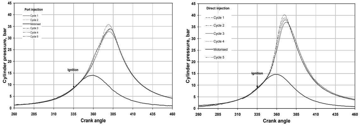
FIGURE 5. Cylinder Pressures of Methane PI (left) and SPFI DI (right)
