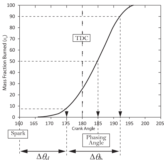
FIGURE 1. Mass Burnt Fraction in A Typical Engine
