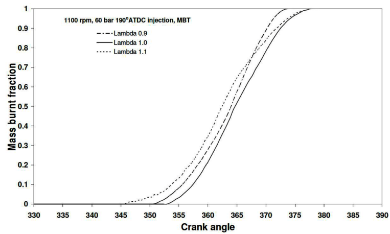
FIGURE 9. Mass Burnt Fraction of Methane SPFI DI at Various Air-Fuel Ratios
