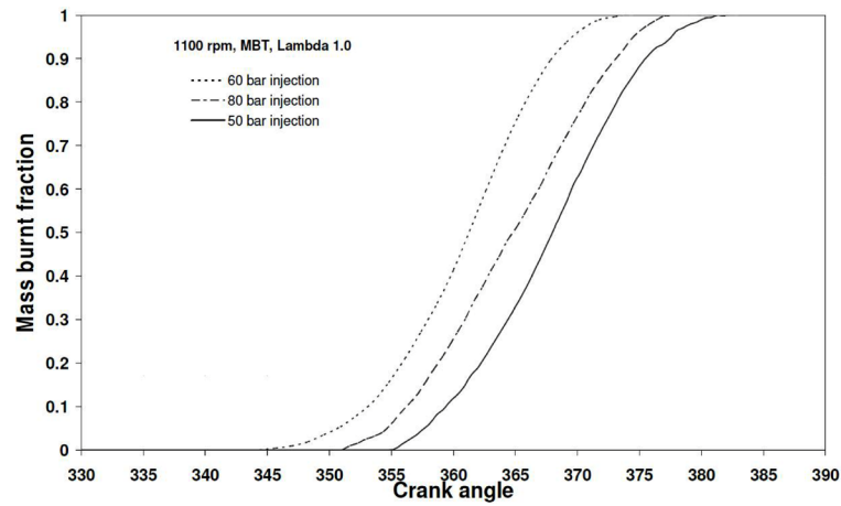
FIGURE 8. Mass Burnt Fraction of Methane SPFI DI at Various Injection Pressures
