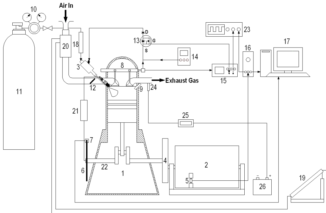
FIGURE 4. Schematic of SPFI Experiment Instrumentation and Data Acquisition System
