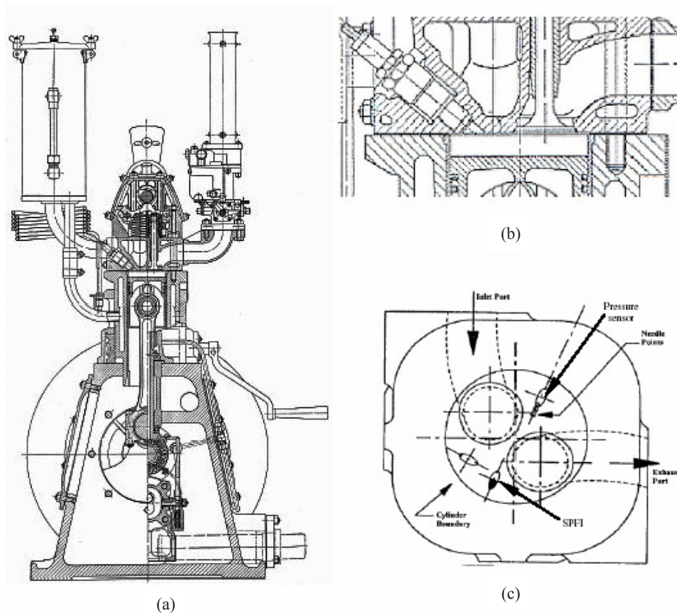
FIGURE 3. Ricardo Single Cylinder Engine; (a) Cross-sectional View of Engine, (b) Cross-sectional View of The Cylinder, (c) Plan View of The Cylinder Head
