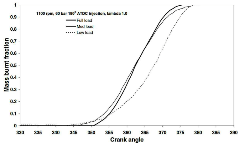
FIGURE 10. Mass Burnt Fraction of Methane SPFI DI at Various Engine Loads
