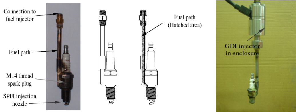
FIGURE 2. Spark Plug Fuel Injector (Left) and Connection to a GDI Injector (Rightmost)
