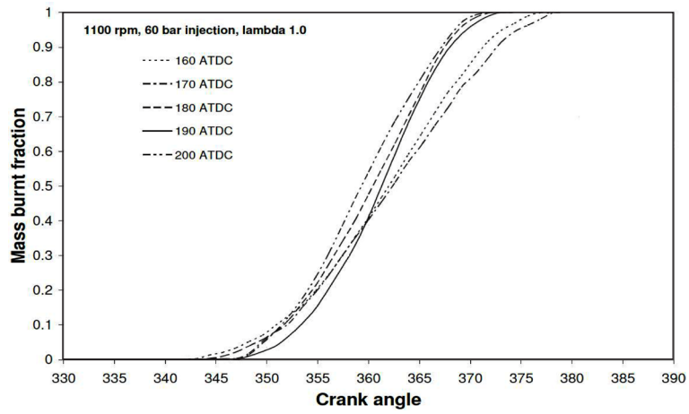
FIGURE 7. Mass Burnt Fraction with Methane SPFI DI at Various Injection Timings
