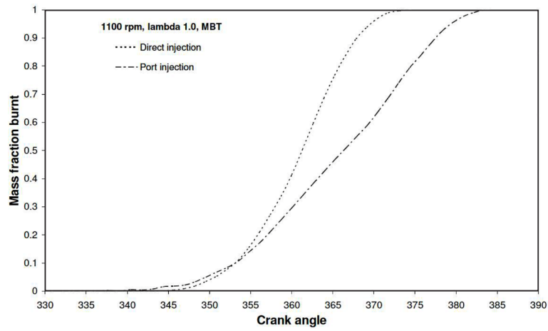
FIGURE 6. Mass Burnt Fractions of Methane PI and SPFI DI
