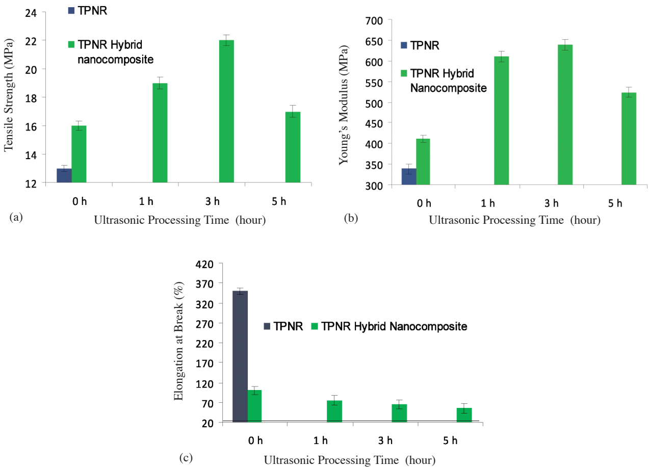
FIGURE 2. Tensile Strength (a), Young's modulus and (b) and Elongation at break (c) of TPNR reinforced with hybrid OMMT-MWNTs
