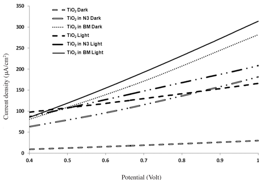
FIGURE 2. The light and dark current density of the TiO 2 photoelectrode in solvent containing the photosensitizer molecule
