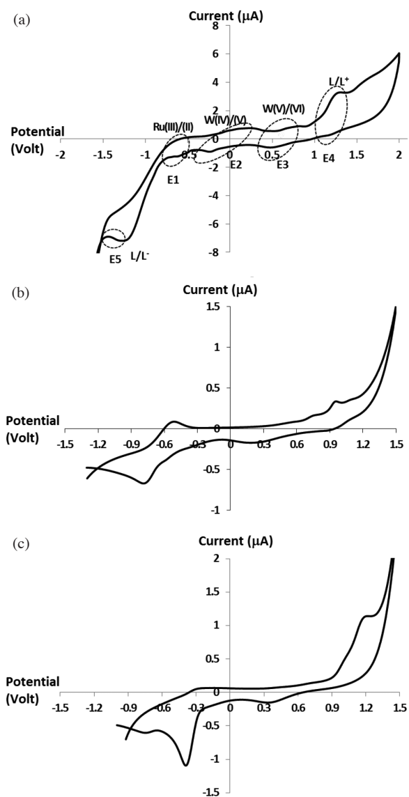
FIGURE 1. The cyclic voltammogram of (a) BM, compared to the monometallic components (b) [Ru(dmtbp) 2 NCS 2 ] and (c) [W(S 2 C 2 Ph 2 ) 2 (CO) 2 ] in DMF/( 1 \times 10^{-4} M) with TBAPF 6 supporting electrolyte. Ag/AgCl was used as the reference and the scan rate was 0.1 \text{ V s}^{-1}
