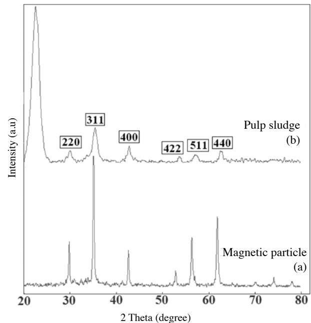
FIGURE 3. X-Ray diffractograms of magnetic particle \text{Fe}_3\text{O}_4 (a) from pulp sludge (b) for IS6
