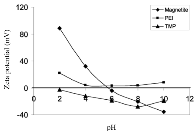
FIGURE 6. Zeta potential of magnetite, PEI and TMP fibre as a function of pH
