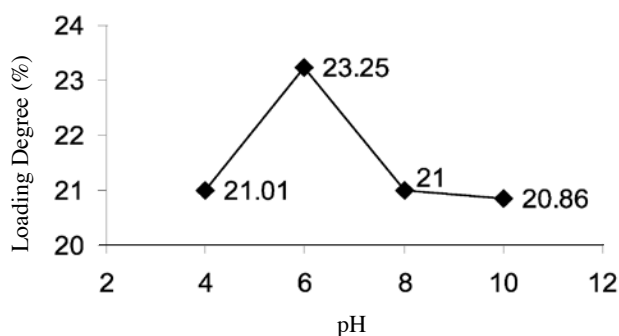
FIGURE 5. Effect of pH on the degree of loading of the magnetic paper
