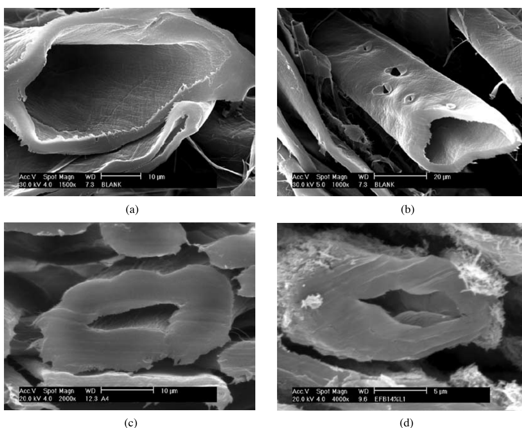
FIGURE 1. Scanning electron micrographs of TMP lumens fiber (a), TMP pits fiber (b), mixed tropical lumens fiber (c) (Ainun 2006) and efb lumens fiber (d) (Humaizah 2002)
