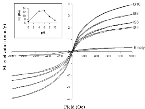
FIGURE 4. Hysteresis loops of the in situ synthesis magnetic papers. The inset figures represent the effects of pH on coercive force, Hc
