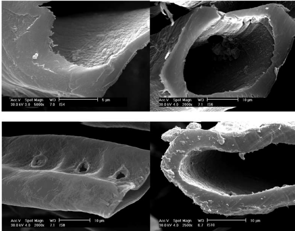
FIGURE 2. Scanning micrograph of magnetic fibers, (acidic condition, IS4 & IS6: alkaline condition, IS8 & IS10)
